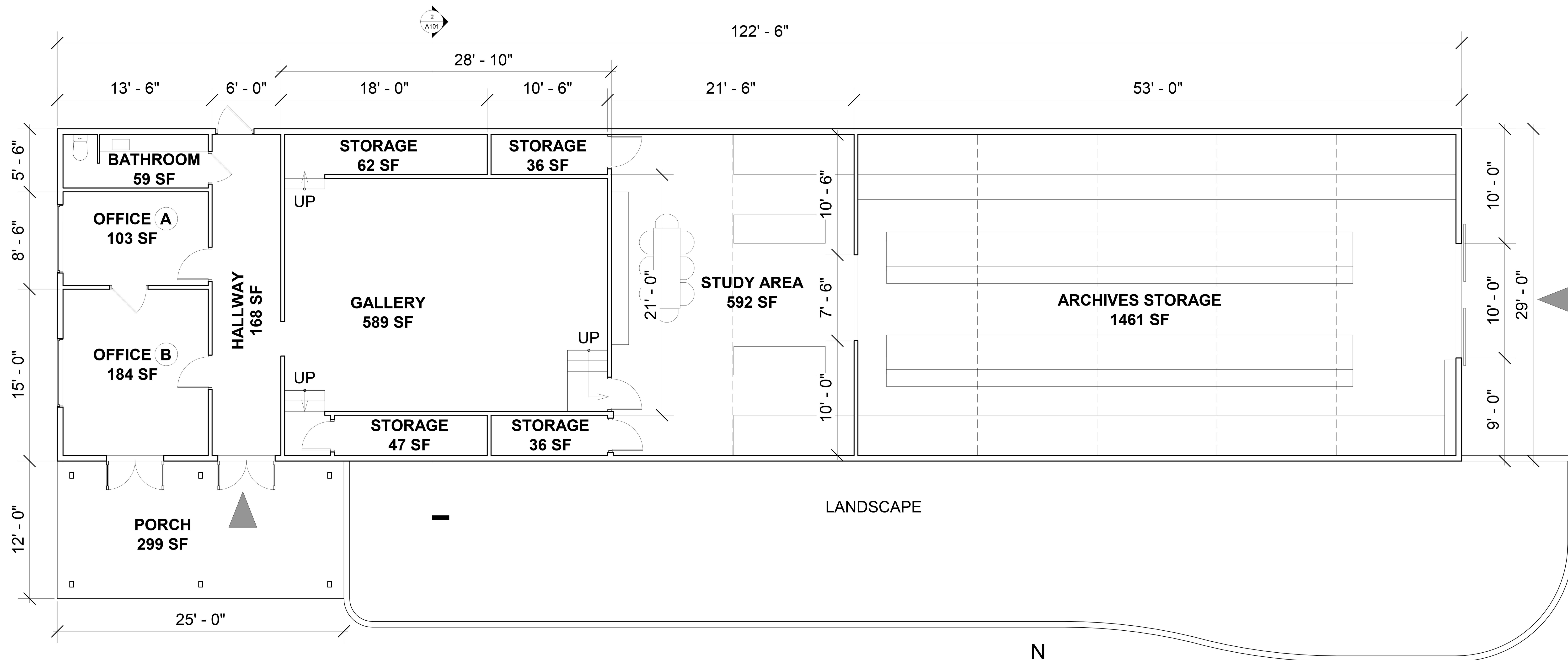
1 1ST FLOOR SPLIT - LEVEL PLAN WARNECKE INSTITUTE ARCHIVES BLDG., SONOMA 1/4"=1'-0"
