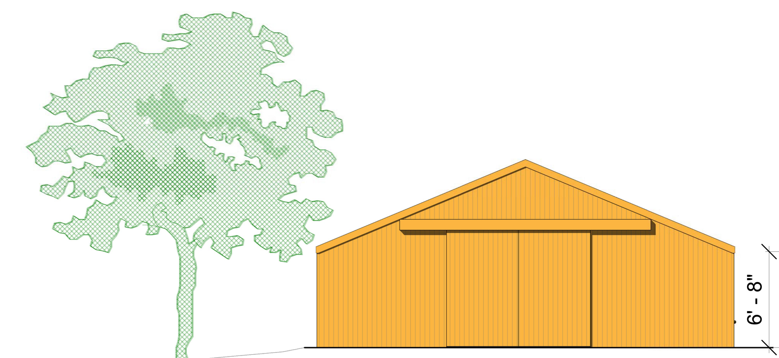
3 EAST ELEVATION WARNECKE INSTITUTE ARCHIVES BLDG., SONOMA 1/4"=1'-0
