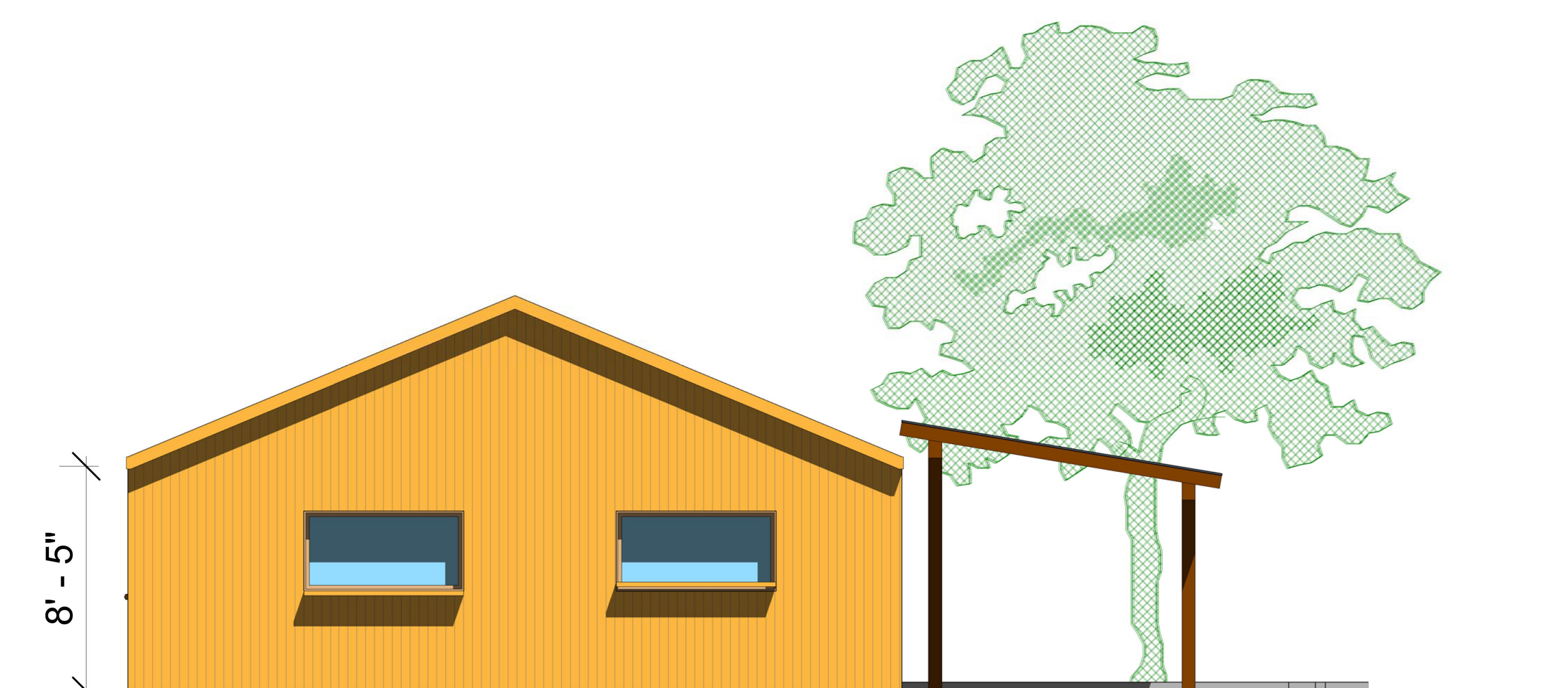
4 WEST ELEVATION WARNECKE INSTITUTE ARCHIVES BLDG., SONOMA 1/4"=1'-0
